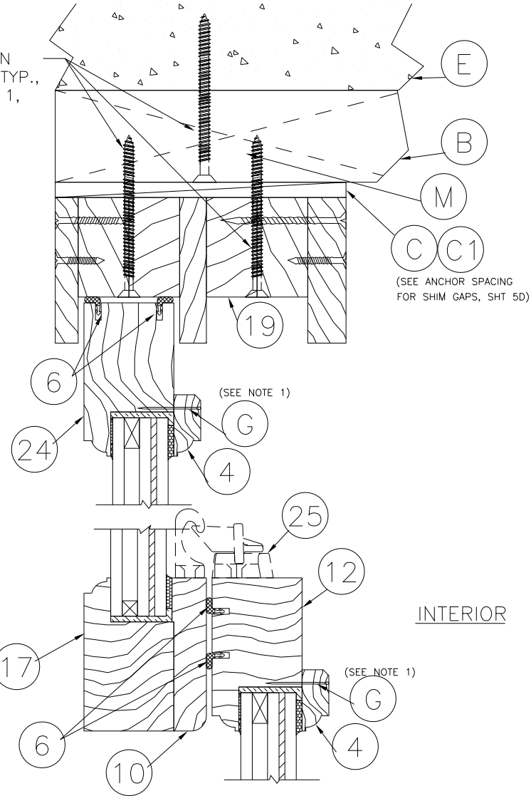
1 3 VERTICAL CROSS SECTION 2X Buck Construction (Thru-the-Frame Installation)
