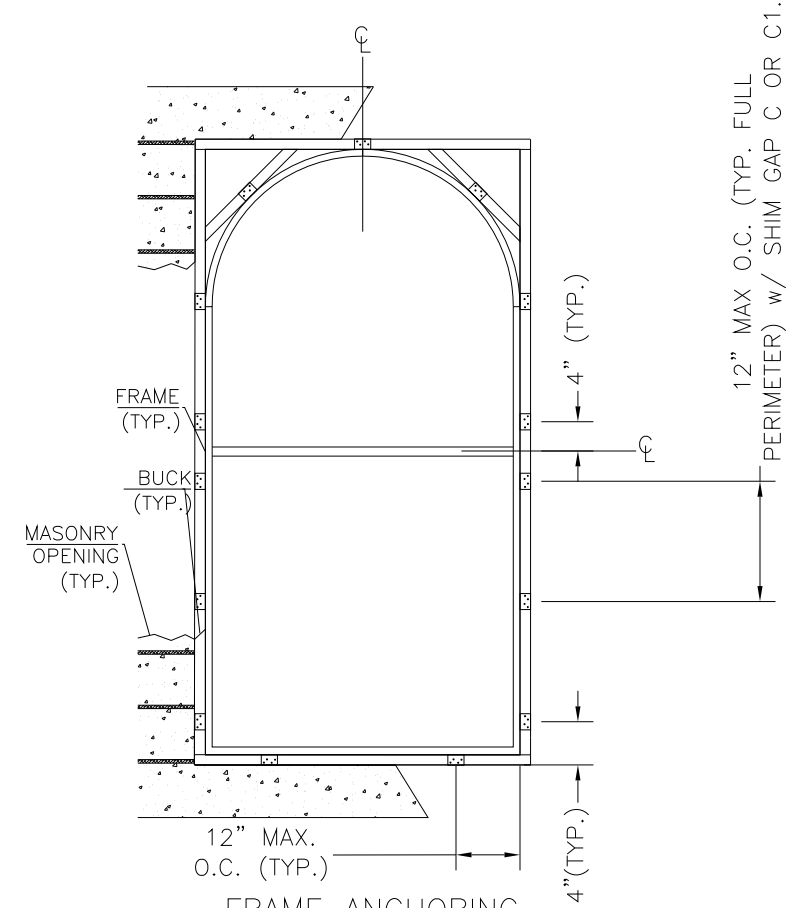
FRAME ANCHORING Anchor Clip Installation
