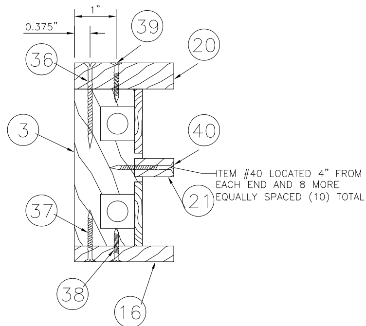
SECTION C-C
