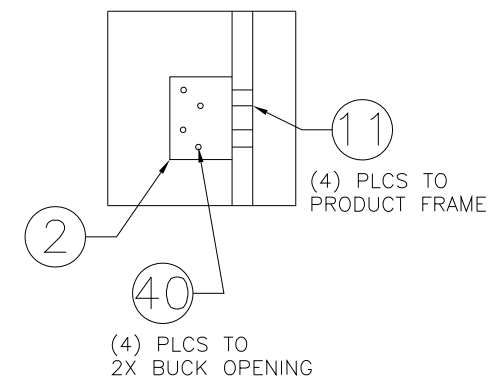
ANCHOR CLIP DETAIL
