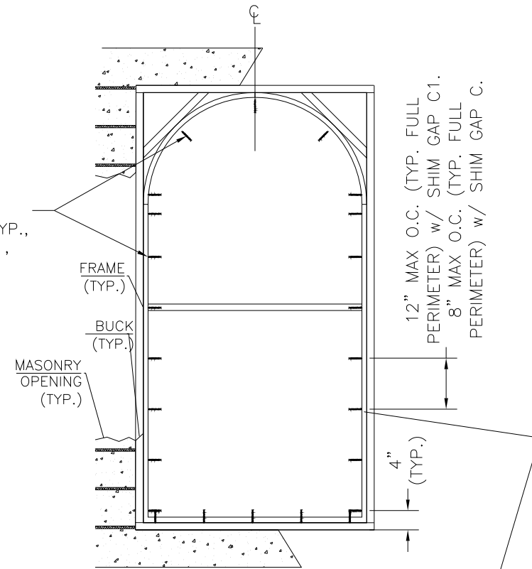
FRAME ANCHORING Through-the-Frame Installation
