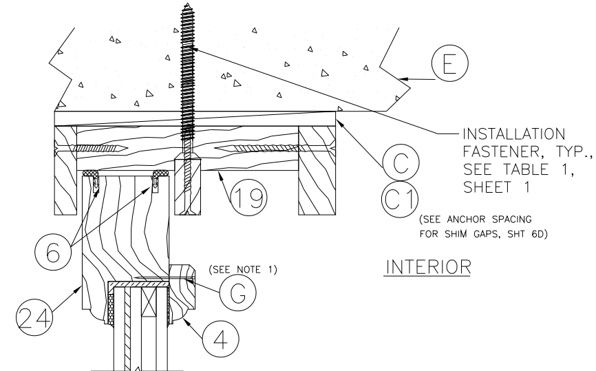
2 4 VERTICAL CROSS SECTION Direct to masonry (Thru-the-Frame Installation)
