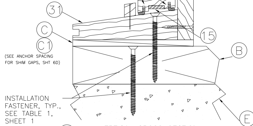
1 4 VERTICAL CROSS SECTION 2X Buck Construction (Thru-the-Frame Installation)
