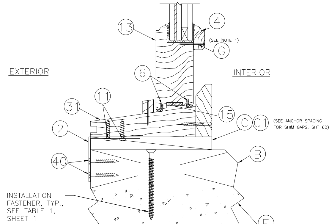
3 4 VERTICAL CROSS SECTION 2X Buck Construction (Anchor Clip Installation)
