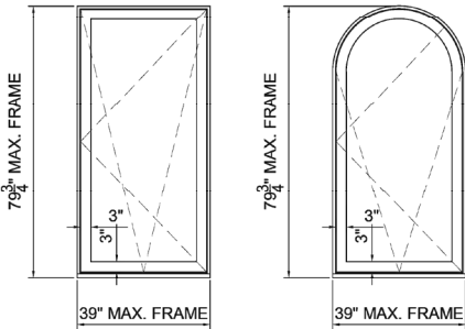
INSWING/TILT&TURN SINGLE CASEMENT WINDOWS
