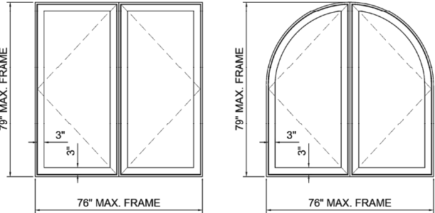
INSWING/OUTSWING TWIN CASEMENT WINDOWS
