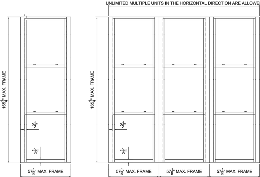
TRIPLE-HUNG SASH WEIGHT AND CHAIN WINDOWS
