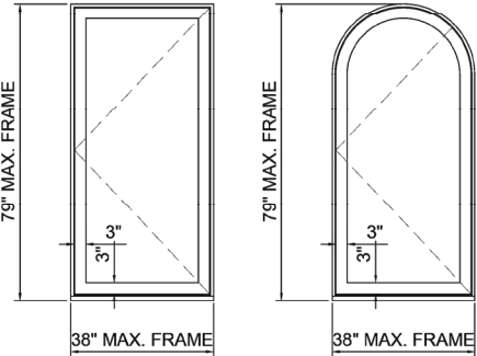
OUTSWING SINGLE CASEMENT WINDOWS
