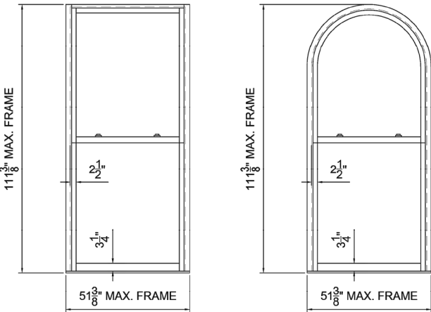
DOUBLE-HUNG BALANCE WINDOWS
