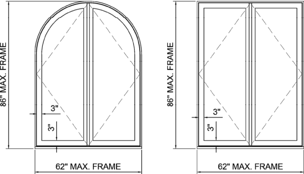
INSWING/OUTSWING FRENCH CASEMENT WINDOWS
