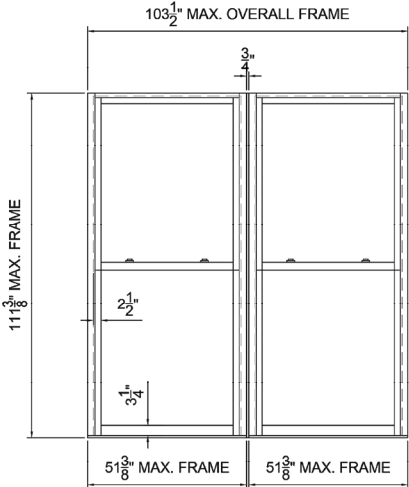
TWIN DOUBLE-HUNG BALANCE WINDOWS
