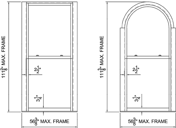
DOUBLE-HUNG SASH WEIGHT AND CHAIN WINDOWS
