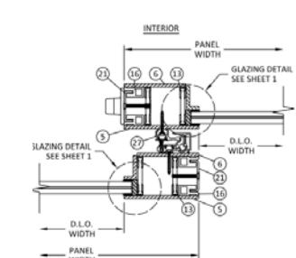
F 6 HORIZONTAL SECTION INTERLOCK
