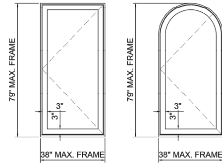
OUTSWING SINGLE CASEMENT WINDOWS
