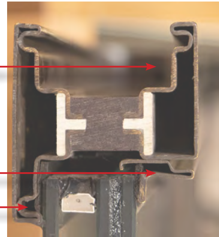
LARGER PROFILE
