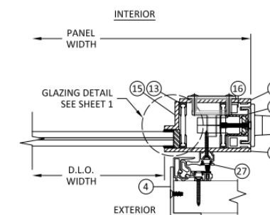
H 6 HORIZONTAL SECTION POCKET JAMB
