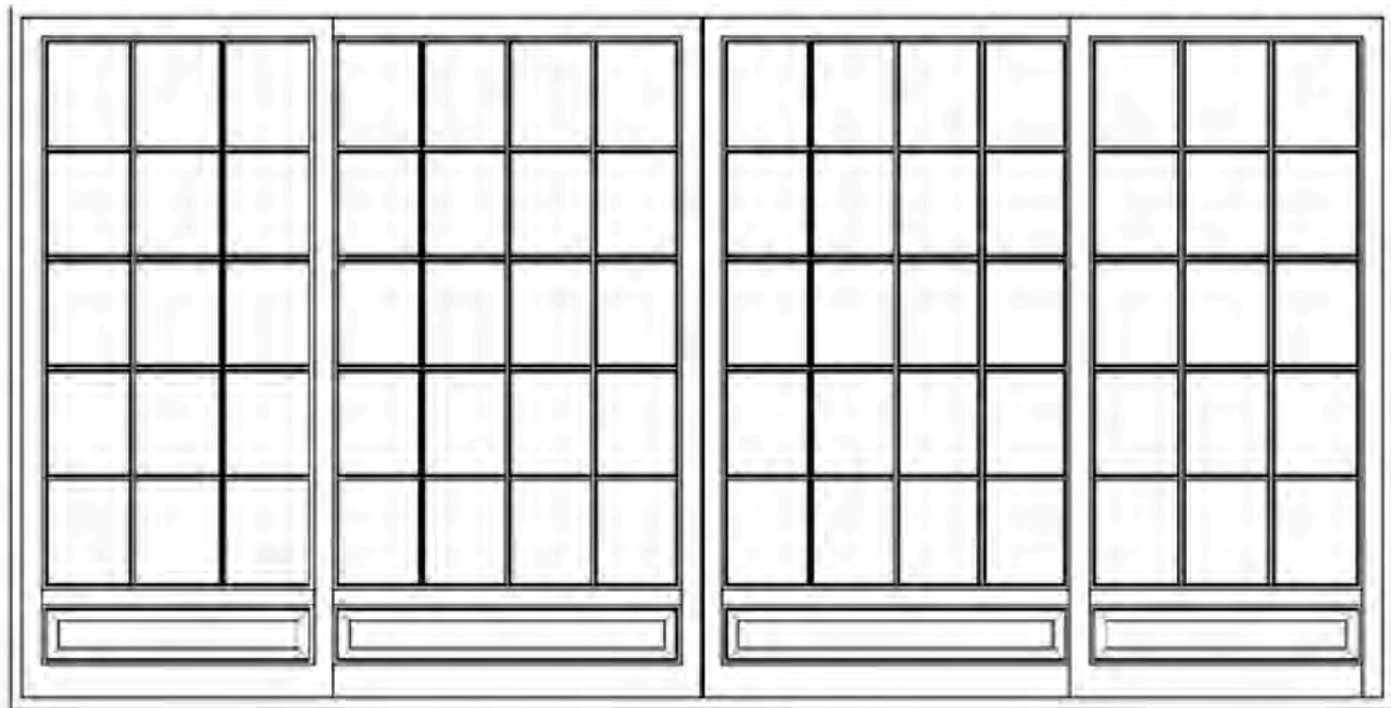
Panel sizes to 5' x 12' Door units to any opening size Design pressures to 60/65 Pocket configuration available
