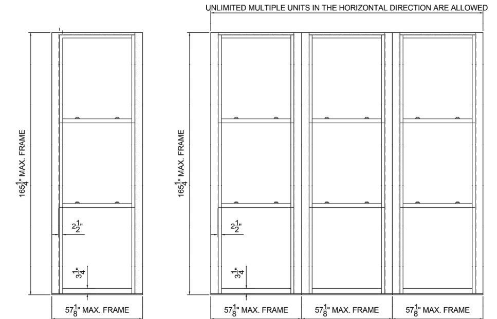
TRIPLE-HUNG SASH WEIGHT AND CHAIN WINDOWS
