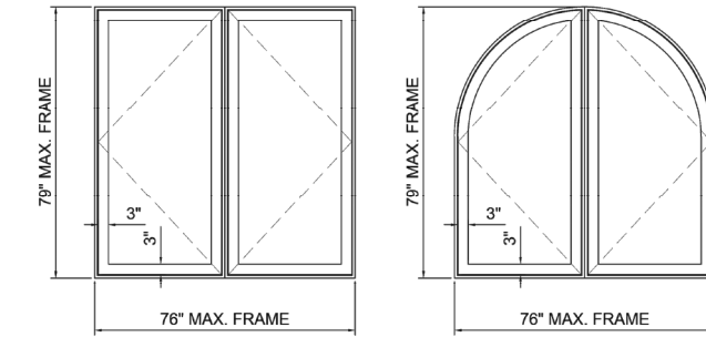
INSWING/OUTSWING TWIN CASEMENT WINDOWS
