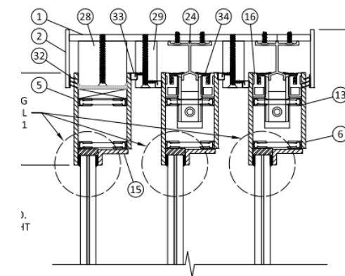
A 4 VERTICAL SECTION DOOR HEAD 3-TRACK
