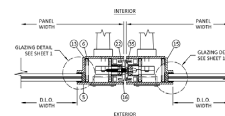
G 6 HORIZONTAL SECTION MEETING STILE
