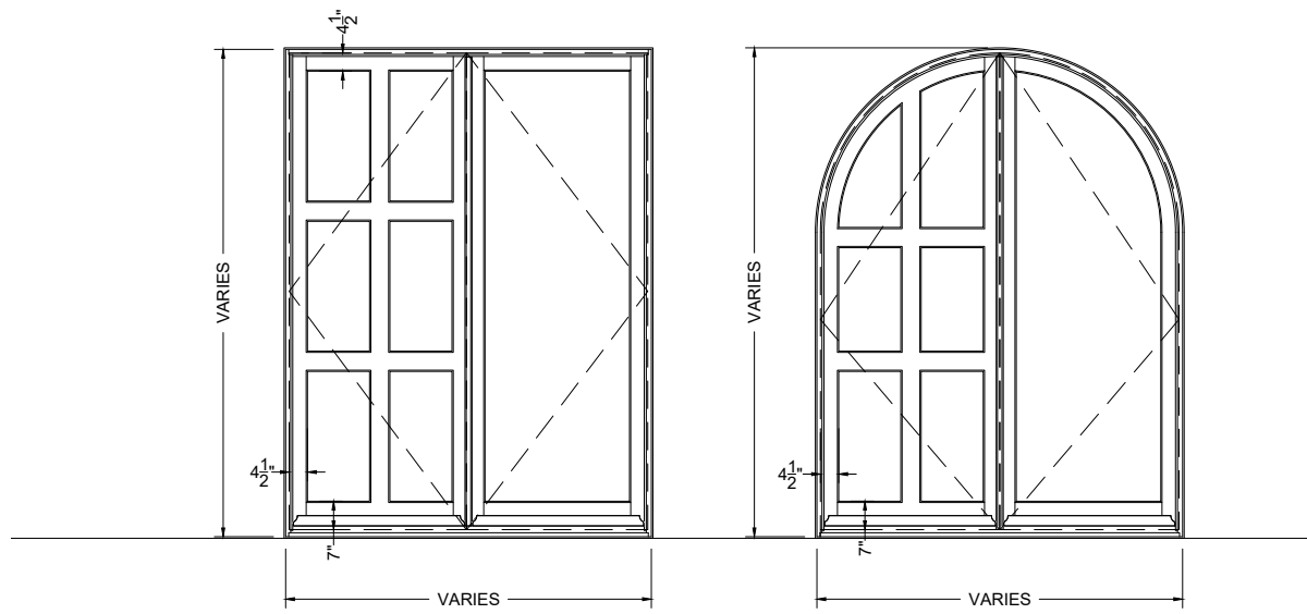
INSWING / OUTSWING 12' DOUBLE DOOR
